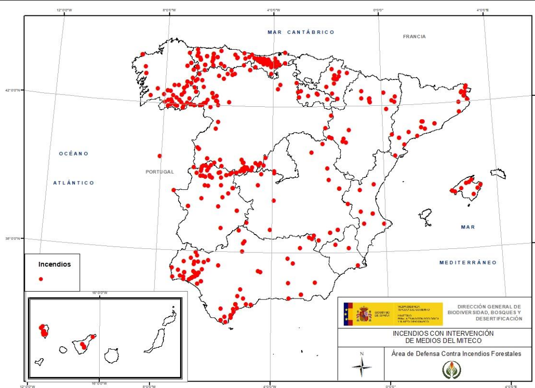
Figure 130. Location of forest fires with the intervention of MITECO means of suppression during 2021.
