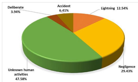
Figure 149. Fire causes in Turkey in 2021.
