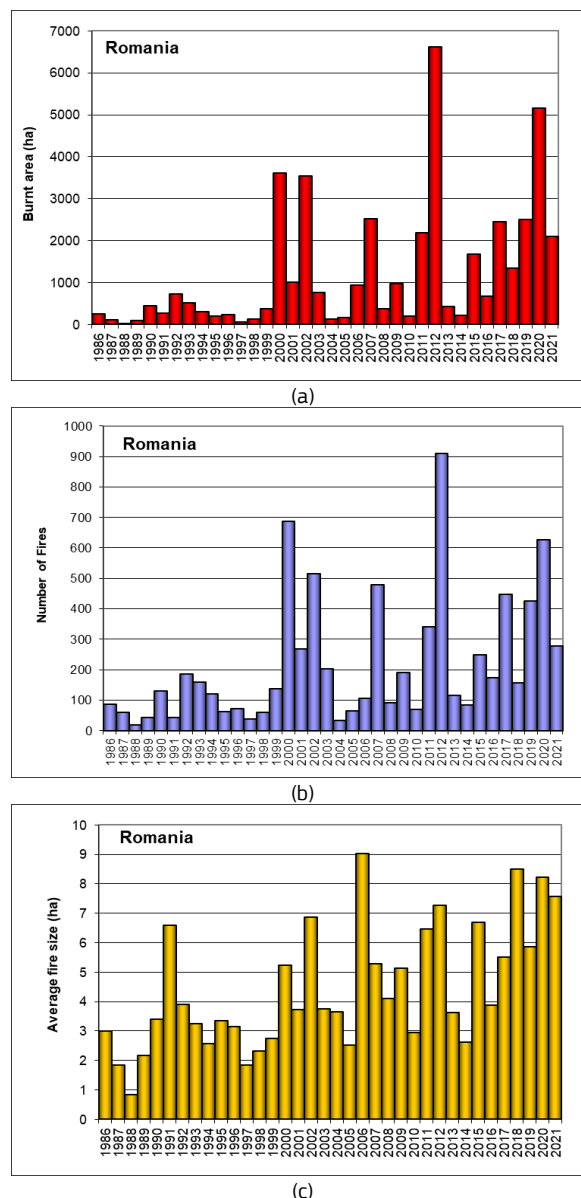
Figure 115. Burnt area (a), number of fires (b) and average fire size (c) in Romania from 1986 to 2021.
