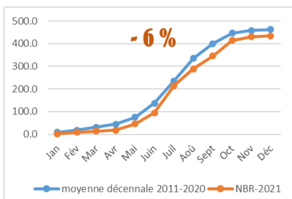
Figure 193. Evolution of number of fires (left) and burnt area (right) in 2021 compared to the last decade.
