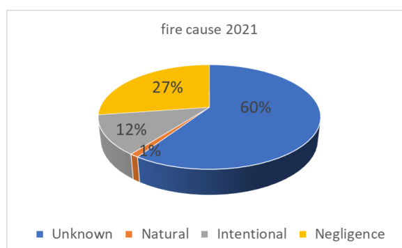
Figure 29. Main causes of wildfire in France in 2021.
