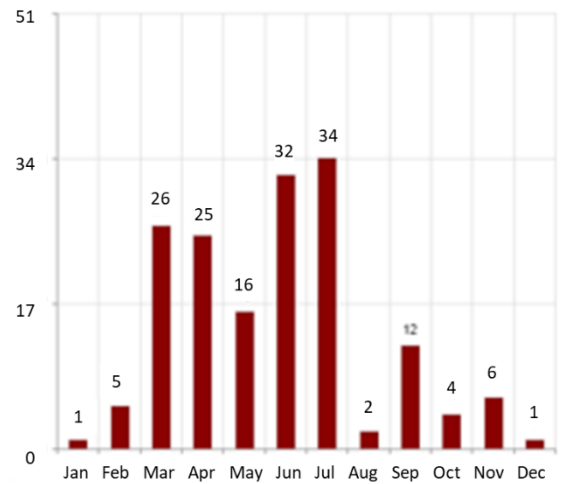
Figure 3. Number of fires by month in Austria in 2021.
