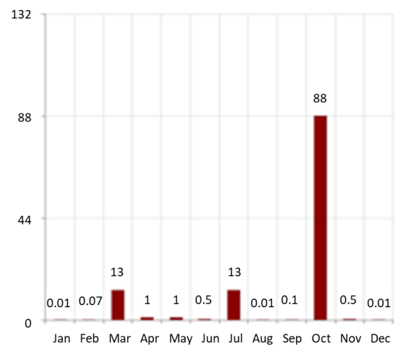
Figure 4. Burnt area in ha by month in Austria in 2021.
