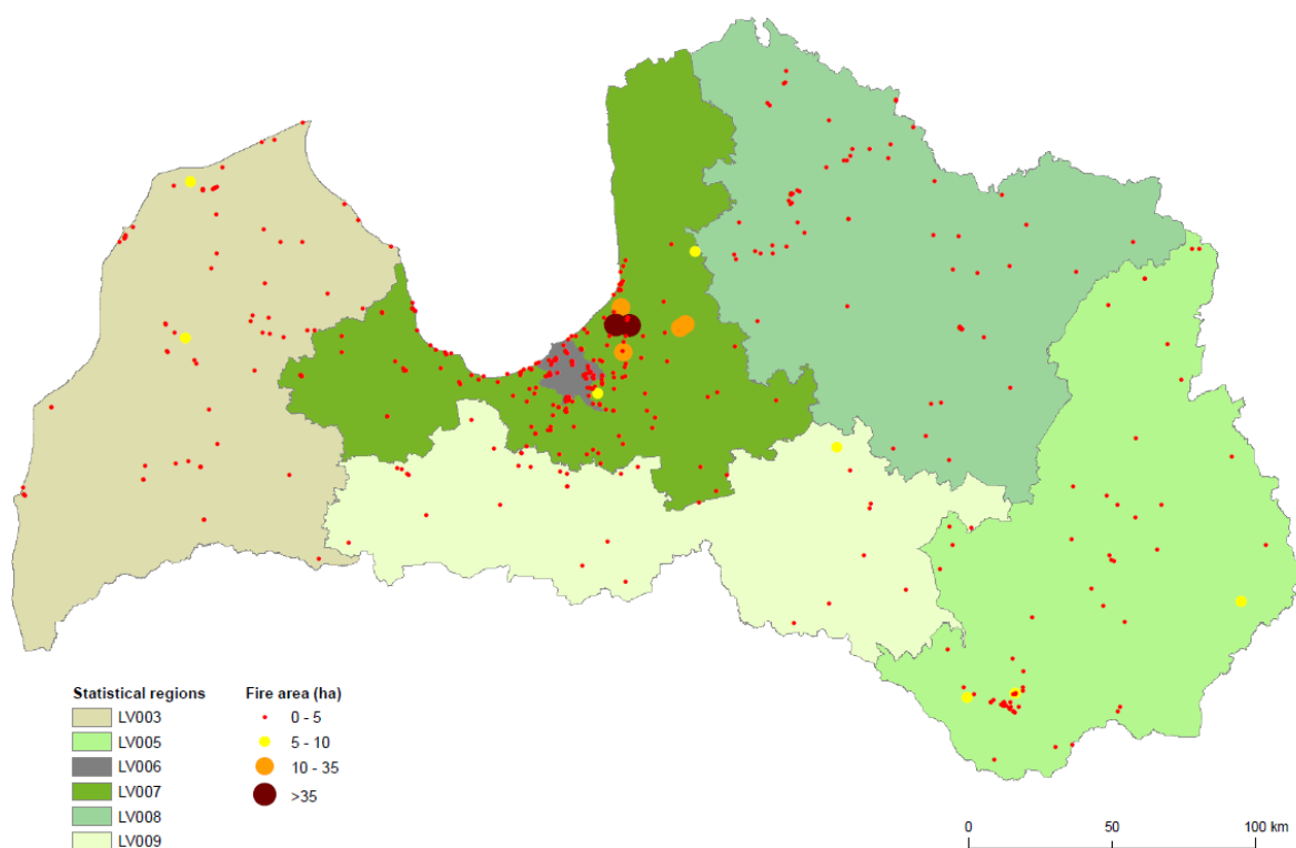
Figure 61. Map of forest fire locations in Latvia in 2021.
